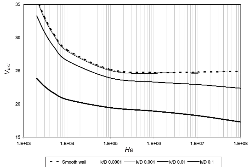
Figure 7. Effect of roughness on transition velocity
