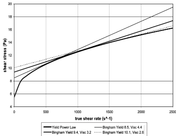
Figure 3. Bingham approximations to yield power law flow curve kaolin SG 1.0803
