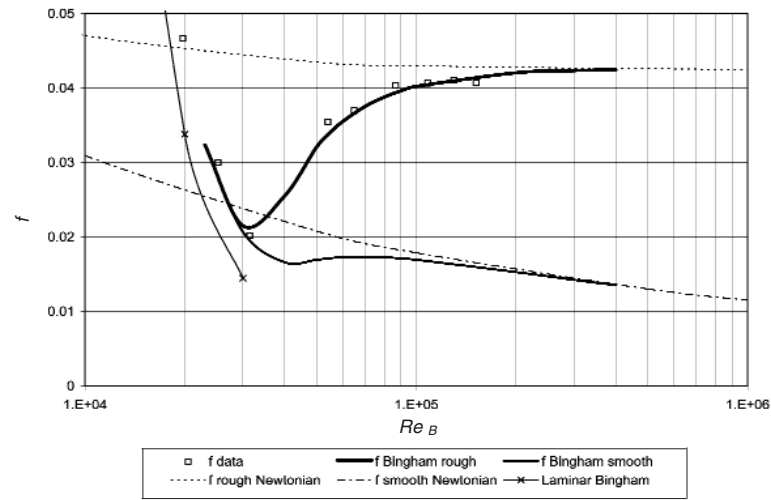
Figure 5. Kaolin rough wall prediction—Bingham yield stress 9.4 Pa
