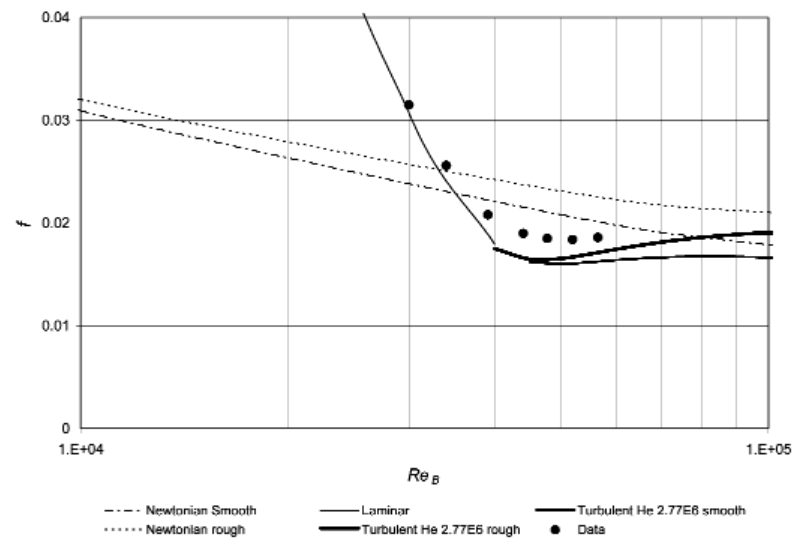
Figure 2. Rough wall prediction compared with limestone data
