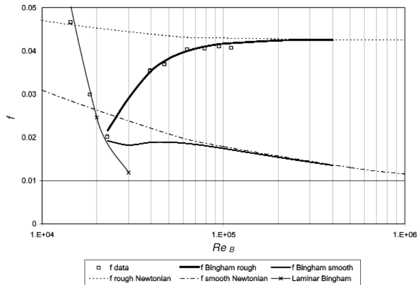
Figure 4. Kaolin rough wall prediction—Bingham yield stress 8.5 Pa
