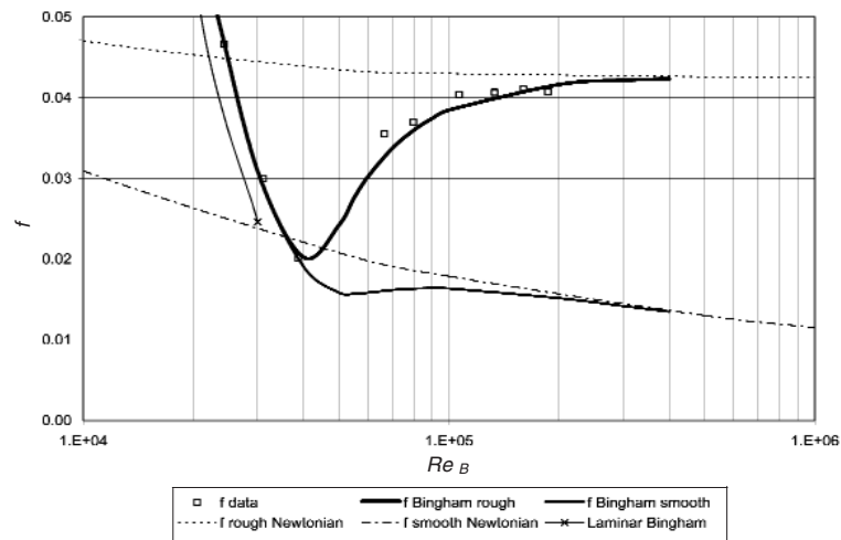
Figure 6. Kaolin rough wall prediction—Bingham yield stress 10.1 Pa
