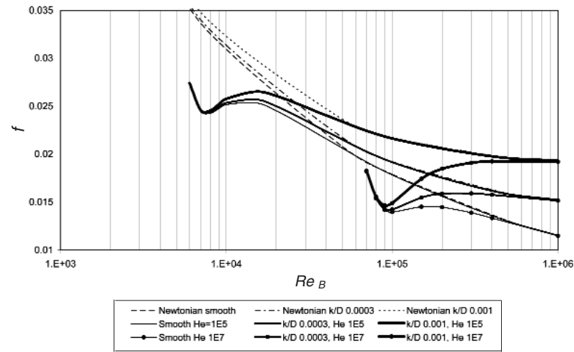
Figure 1. Smooth and rough wall predictions for He = 1E5 and 1E7
