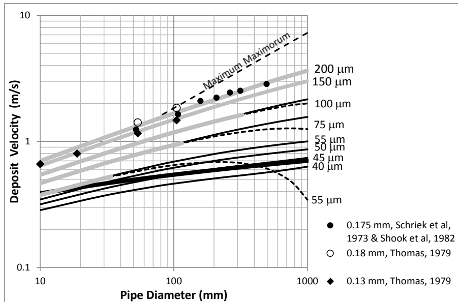
Figure 1 Deposit velocity vs pipe diameter – Comparisons MW&J and W&J predictions
