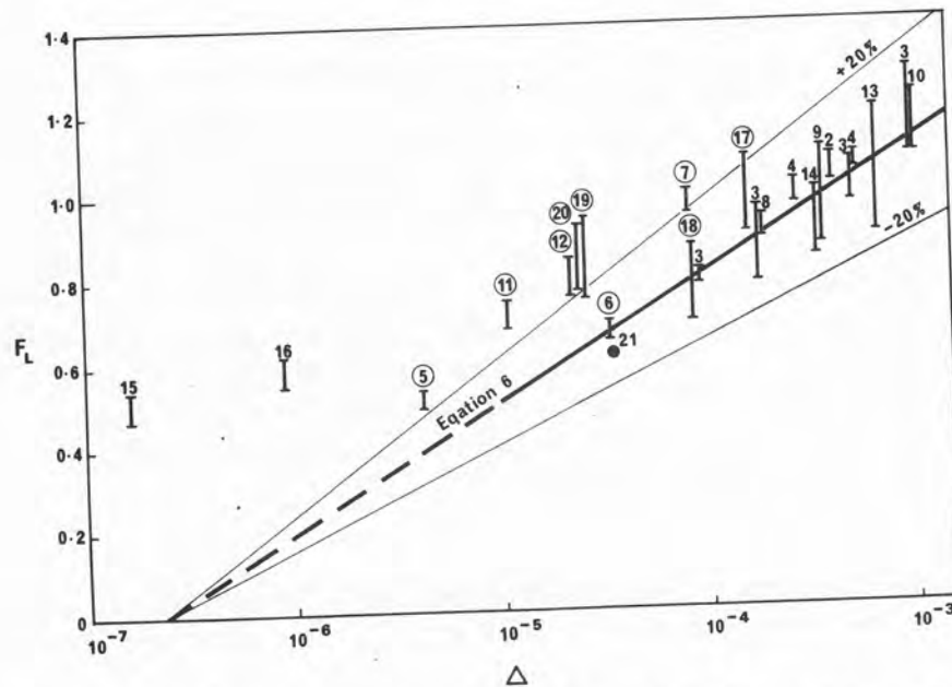
Figure 3. The use of \Delta as a correlating tool. Comparison between [6] and observed values of F_L at deposition for a concentration of 12%. For experimental conditions refer to numbers in tables 1 and 2. Ringed numbers indicate fluid viscosities greater than 1.1 \times 10^{-3} \text{ N s m}^{-2} .
