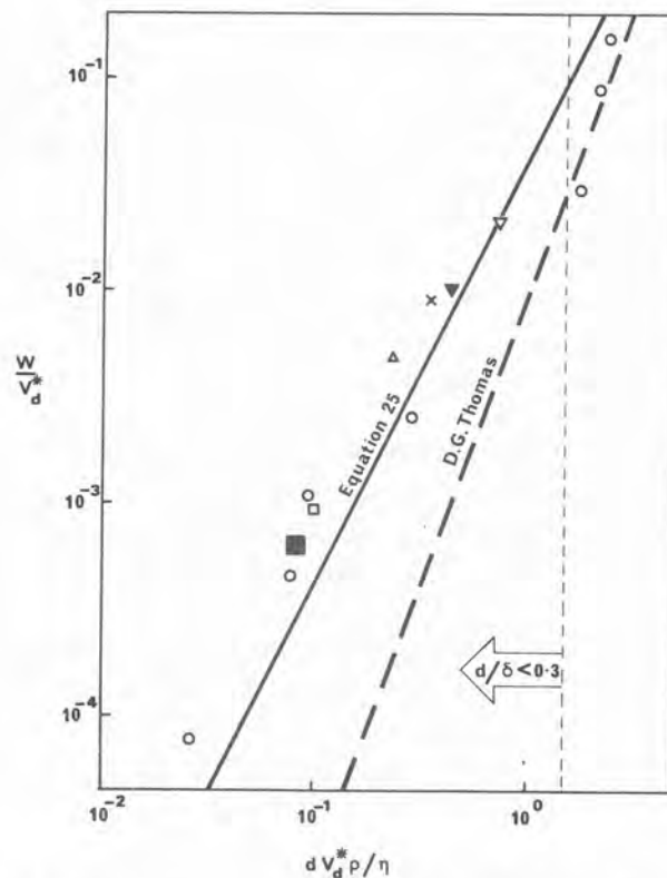
Figure 8. Comparing present viscous sub-layer deposition theory with that of Thomas (1962/2) for flocculated particles. \nabla , 17 \mu\text{m} sand (15); \nabla , 26 \mu\text{m} sand (16); \circ , Thomas' data re-calculated using particle properties; the remaining data from Cairns et al. (1960), \times , 15 \mu\text{m} talc; \square , 3.7 \mu\text{m} barium sulphate; \blacksquare , 2.3 \mu\text{m} lead; \triangle , 4.8 \mu\text{m} tungsten.
